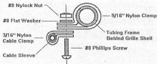
Cable Clamping Assembly - Illustration "C"
